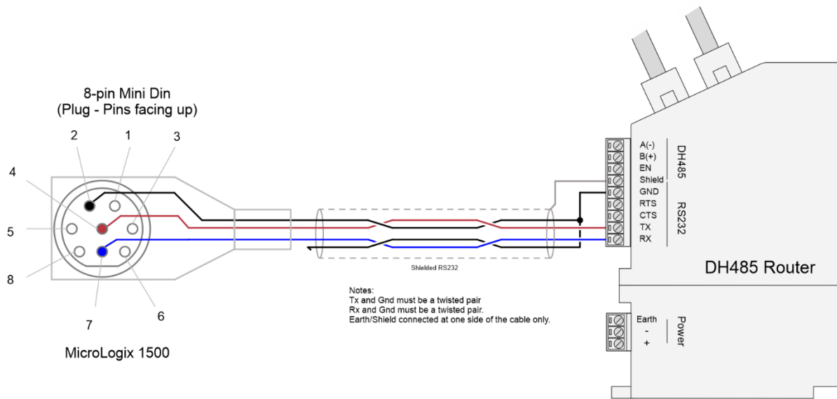
Figure 7.4 – DH485R/B – MicroLogix 1500 (RS232)
