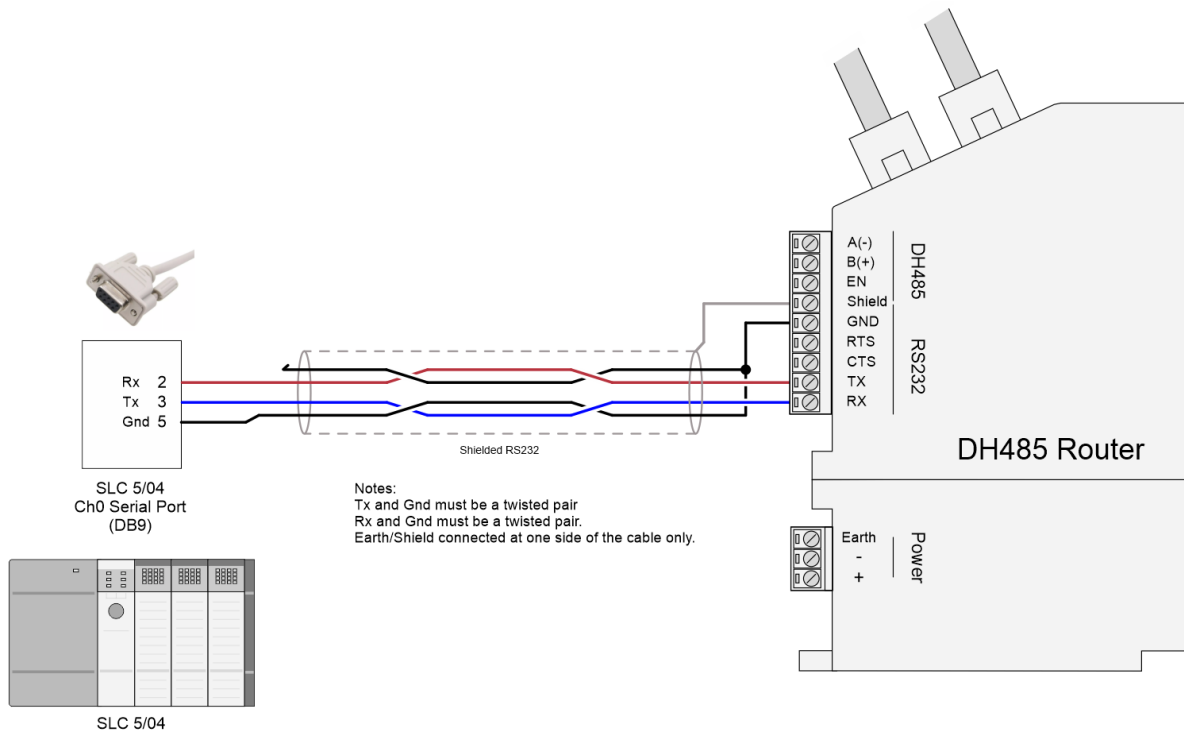
Figure 7.5 – DH485R/B – SLC5/04 (RS232)
