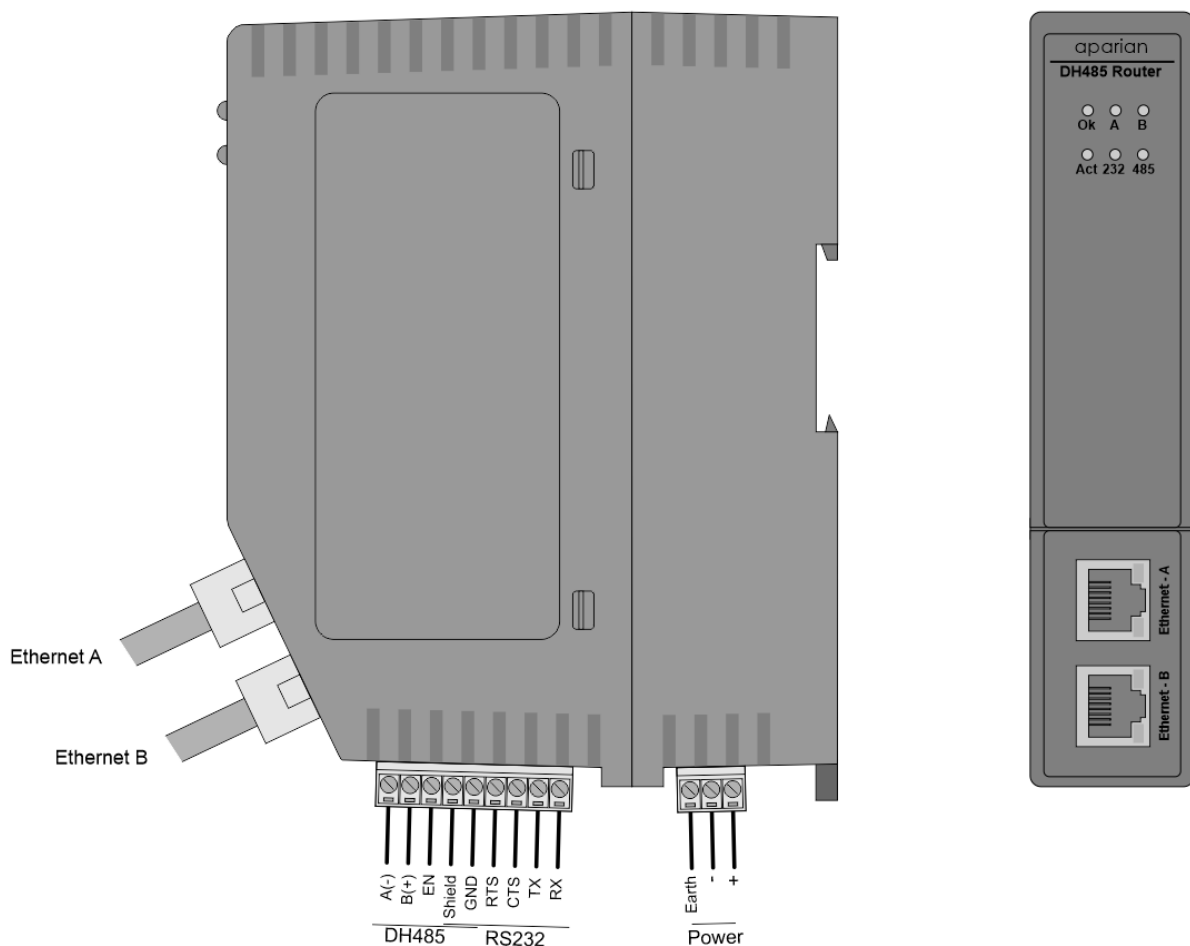
Figure 2.1. - DH485 Router/B side and front view
