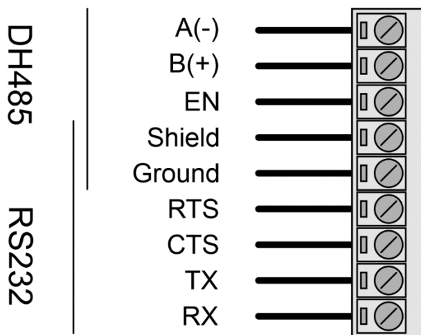
Figure 2.6 - RS232 / DH485 connector
